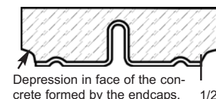
6. After the concrete is poured and cured, remove end caps with screw driver or crow bar. End caps may be replaced to protect sleeve until pipe penetration is made.
